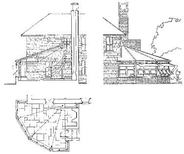
Plan, section, elevation
